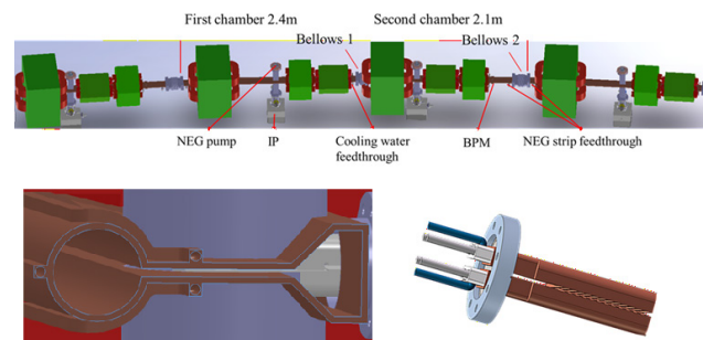
Figure 6: Model of one arc vacuum cell of the collider rings together with the cross-section and a photo absorber under prototyping
