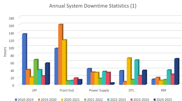
Figure 4: Annual downtime (hours) by system (a).
