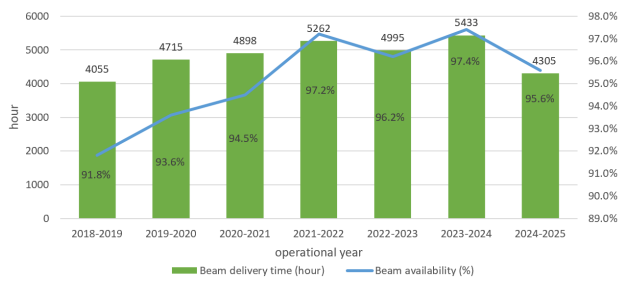
Figure 3: Delivered Beam Time and Beam Availability by Operational Year.
