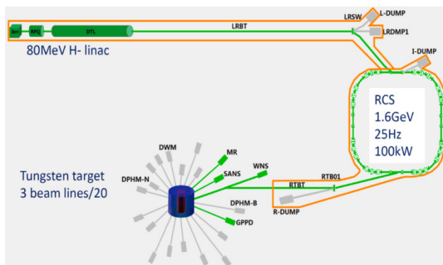
Figure 1: Schematic layout of CSNS.
