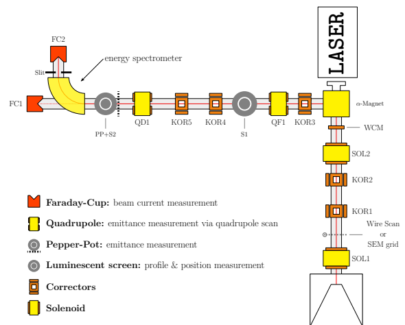
Figure 5: Initial concept of the gun test stand. Dimensions are not to scale.
