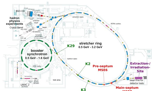
Figure 1: Accelerator facility ELSA with the marked locations of the injection kickers in green, pre- and main-septum in red and the FLASH experimental site in purple.
