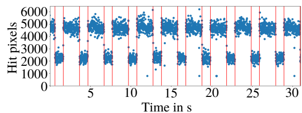
Figure 4: Number of registered pixel hits during a measurement in storage mode . The reconstructed time slices for analysis are indicated in red. The change in the hit rate with and without laser radiation is clearly visible.
