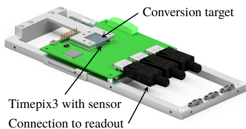
Figure 3: Image of the Timepix3 detector. The Timepix 3 with the 500 \mu\text{m} sensor is hidden under the target.
