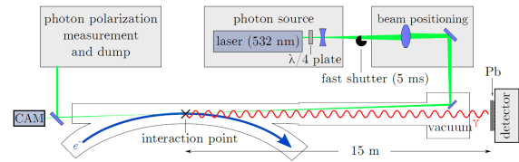
Figure 1: Principle setup of the Compton backscattering polarimeter at ELSA [4].
